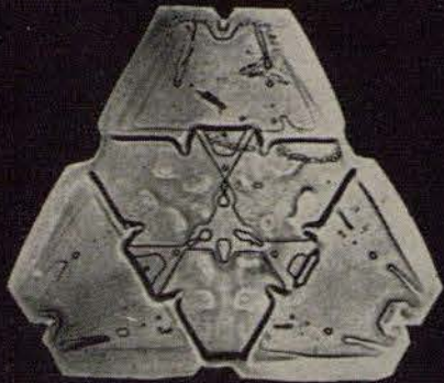
TRIANGLE CRYSTALS (UPPER LEFT) ARE RARE. ALL OTHER CRYSTALS ARE HEXAGONAL
