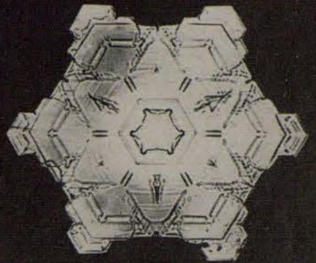
FROM HEXAGON (UPPER LEFT), CRYSTALS PROGRESS INTO MORE ELABORATE PATTERNS
