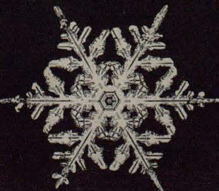
THESE CRYSTALS, BUILT UP IN WARM TEMPERATURE, HAVE THIN, DELICATE SPOKES
