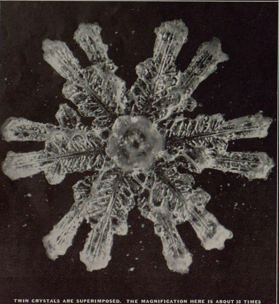
TWIN CRYSTALS ARE SUPERIMPOSED. THE MAGNIFICATION HERE IS ABOUT 30 TIMES
