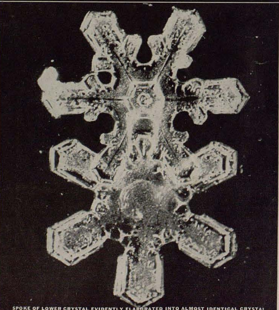
SPOKE OF LOWER CRYSTAL EVIDENTLY ELABORATED INTO ALMOST IDENTICAL CRYSTAL
