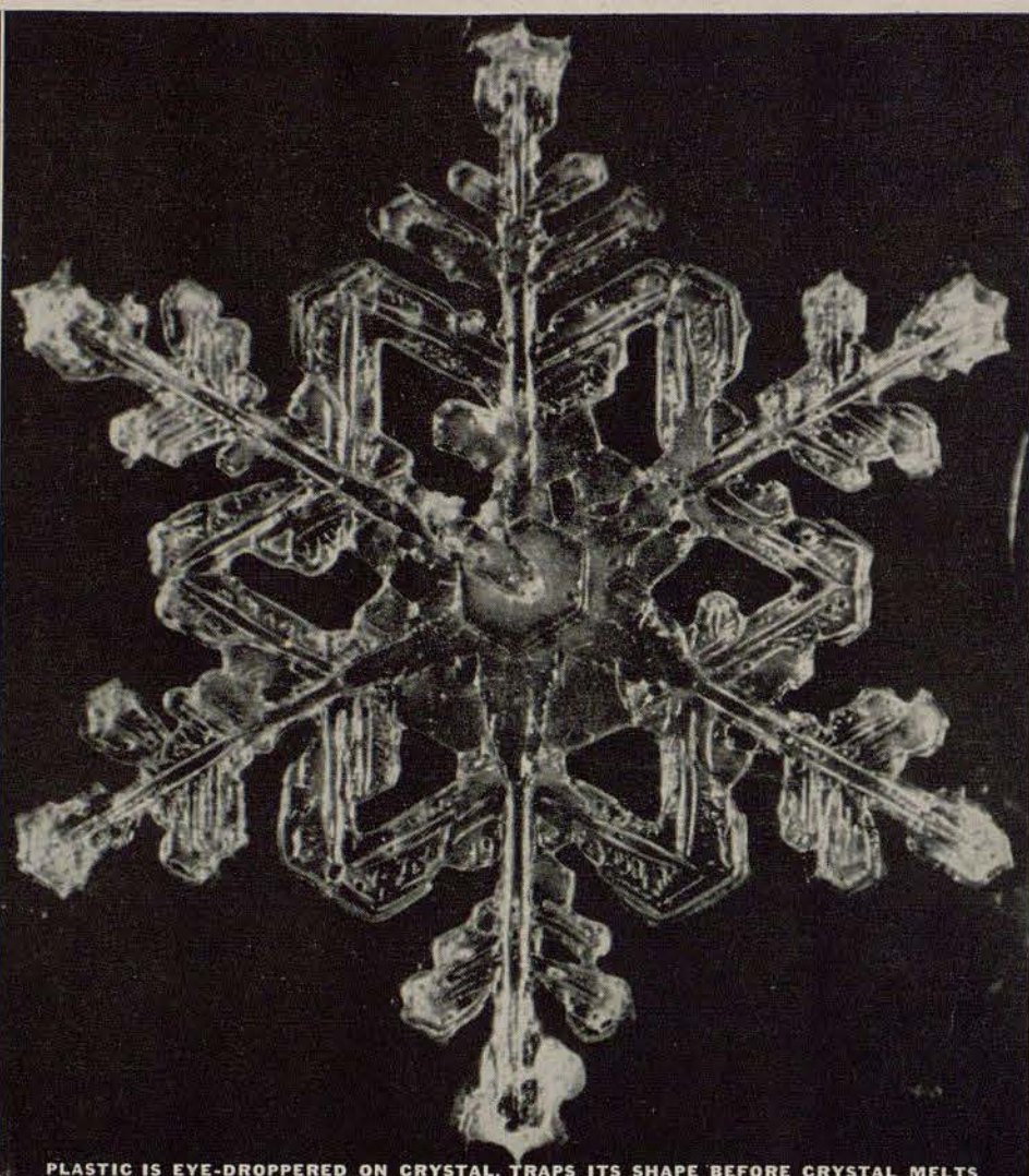
PLASTIC IS EYE-DROPPED ON CRYSTAL, TRAPS ITS SHAPE BEFORE CRYSTAL MELTS
