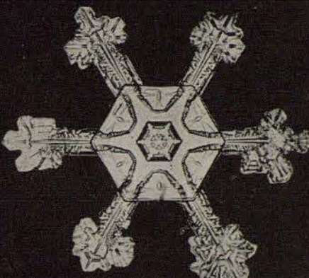
FROM HEXAGON (UPPER LEFT), CRYSTALS PROGRESS INTO MORE ELABORATE PATTERNS
