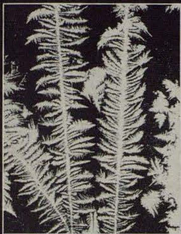
IN SPRING AND AUTUMN, RIME INCRYSTALS LEAVES AND GRASS-BLADES
