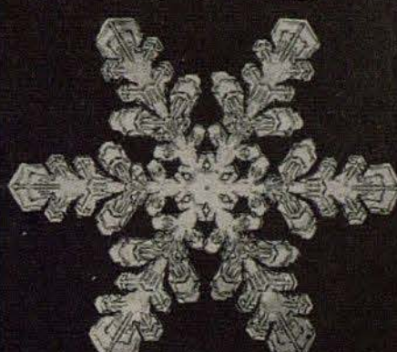
AROUND TINY CENTRAL HEXAGONS CRYSTALS DEVELOP ELABORATE GOTHIC SPOKES
