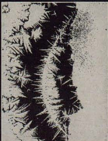
INDOOR HUMIDITY FROSTS WINDOWPANES WITH LUSH TROPICAL FORESTS
