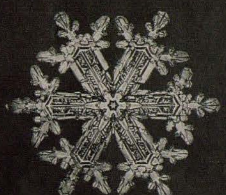
AROUND TINY CENTRAL HEXAGONS CRYSTALS DEVELOP ELABORATE GOTHIC SPOKES
